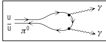
Figure 1. The decay of \pi^0 according to the quark model.
